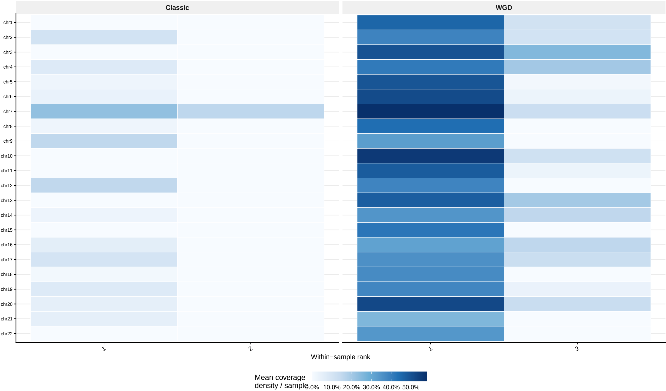
Chromosome coverage density by class × clock rank Colour = sum(seg length) / chr length / n_samples | Stars = Wilcoxon vs row median (BH)
